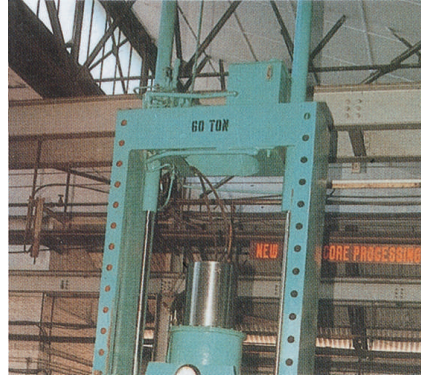
Vertical press installed for accurate rotor core building.
