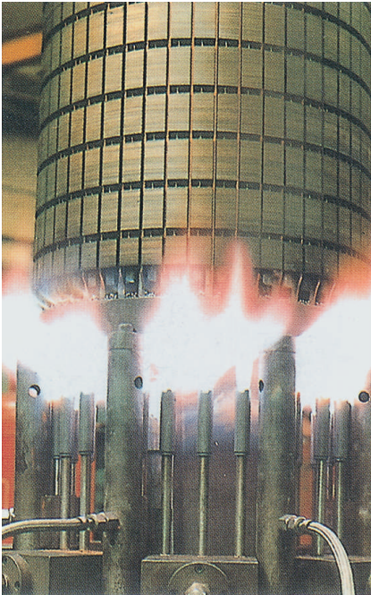
One shot Rotor brazing
