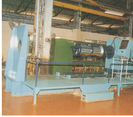
Core Insertion Machine installed for insertion of wound core into frame.
