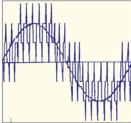
Fig. 1 Typical sine wave generated by inverter pulse
