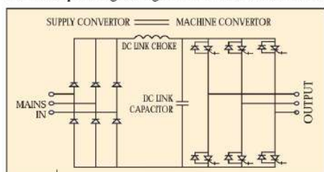
Fig. 2 Typical Voltage Source PWM inverter
